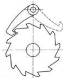
Sperrhaken
